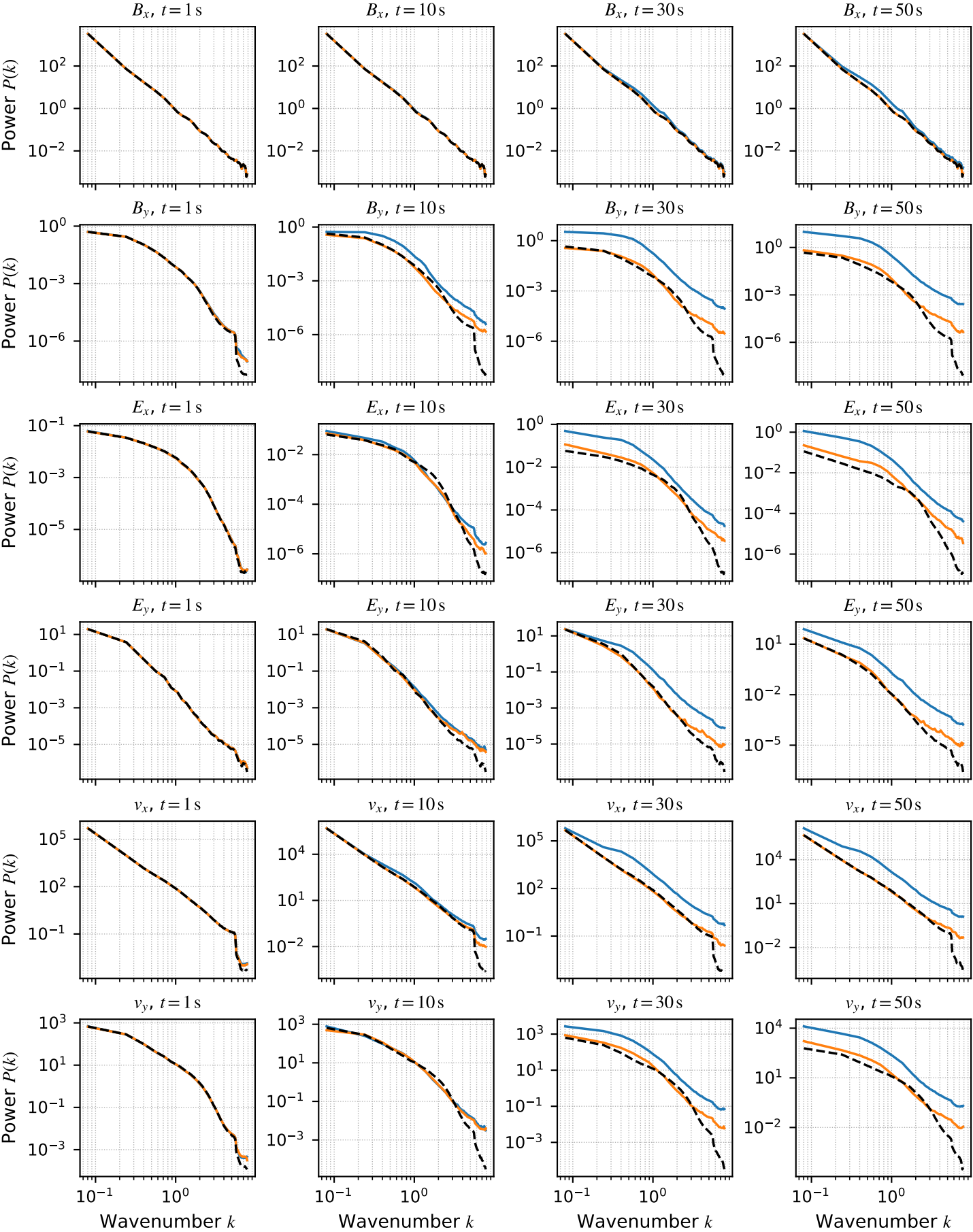
— Graph-FM — Graph-EFM - - - Vlasiator
