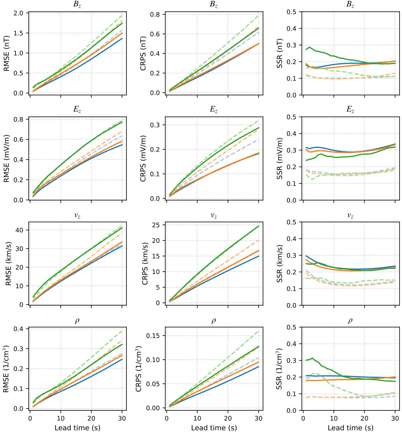
-- Graph-EFM (simple, before \mathcal{L}_{\text{CRPS}} ) -- Graph-EFM (multiscale, before \mathcal{L}_{\text{CRPS}} ) -- Graph-EFM (hierarchical, before \mathcal{L}_{\text{CRPS}} ) — Graph-EFM (simple, \lambda_{\text{CRPS}} = 10^6 ) — Graph-EFM (multiscale, \lambda_{\text{CRPS}} = 10^6 ) — Graph-EFM (hierarchical, \lambda_{\text{CRPS}} = 10^5 )
